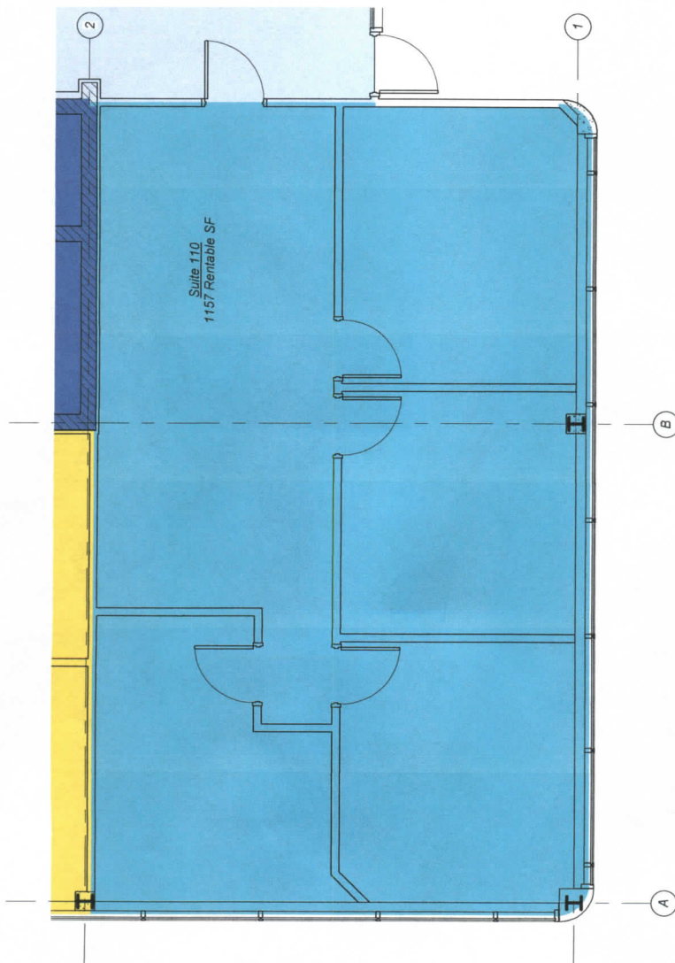
1 110 FIRST FLOOR- SUITE 110 SCALE: 3/16" = 1'-0"
